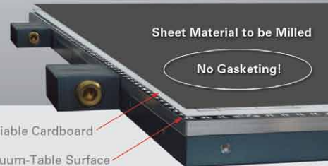
Vacuum Table / Vacuum Chuck
